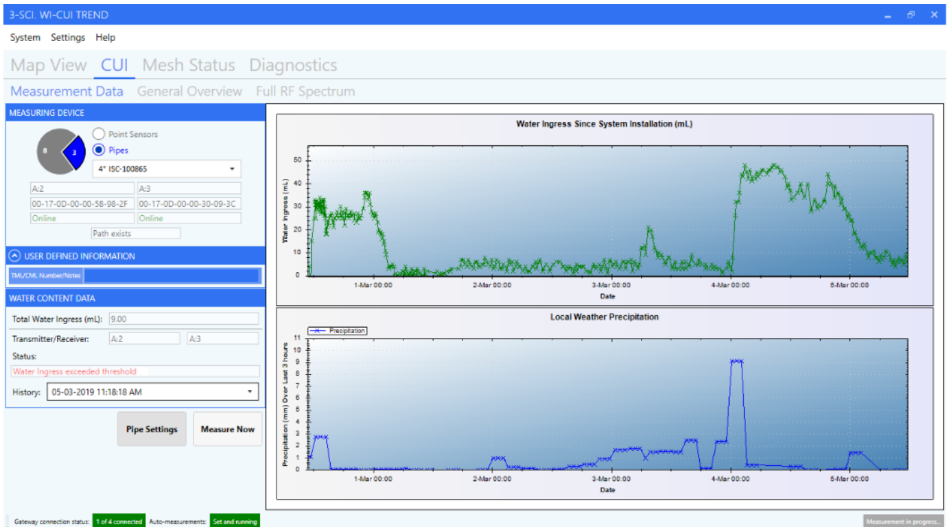
Wi-Corr user interface showing a correlation between water ingress into the insulation due to metal cladding leaks and local rainfall
